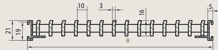
392/1 Linear bar louvre with L frame without flange
