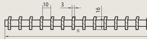
392/3: Linear bar louvre without frame
