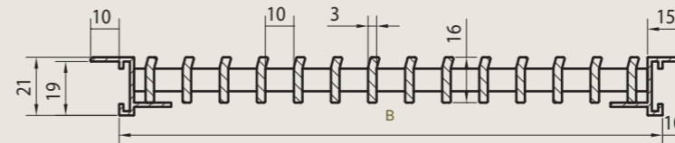
392/2: Linear bar louvre with Z frame with flange
