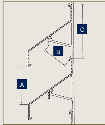
A. Visual distance between two blades B. Narrowest gap between two blades C. Blade pitch
