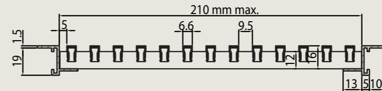
394/2: Linear bar louvre with frame with flange
