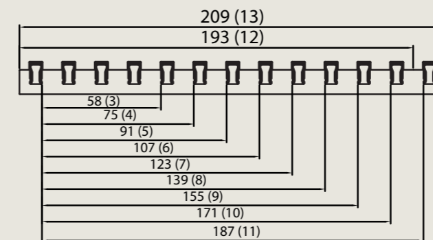
394/3: Linear bar louvre without frame
