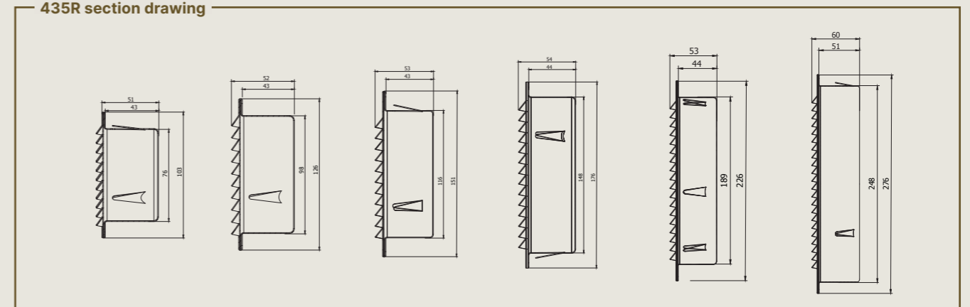
435R section drawing
