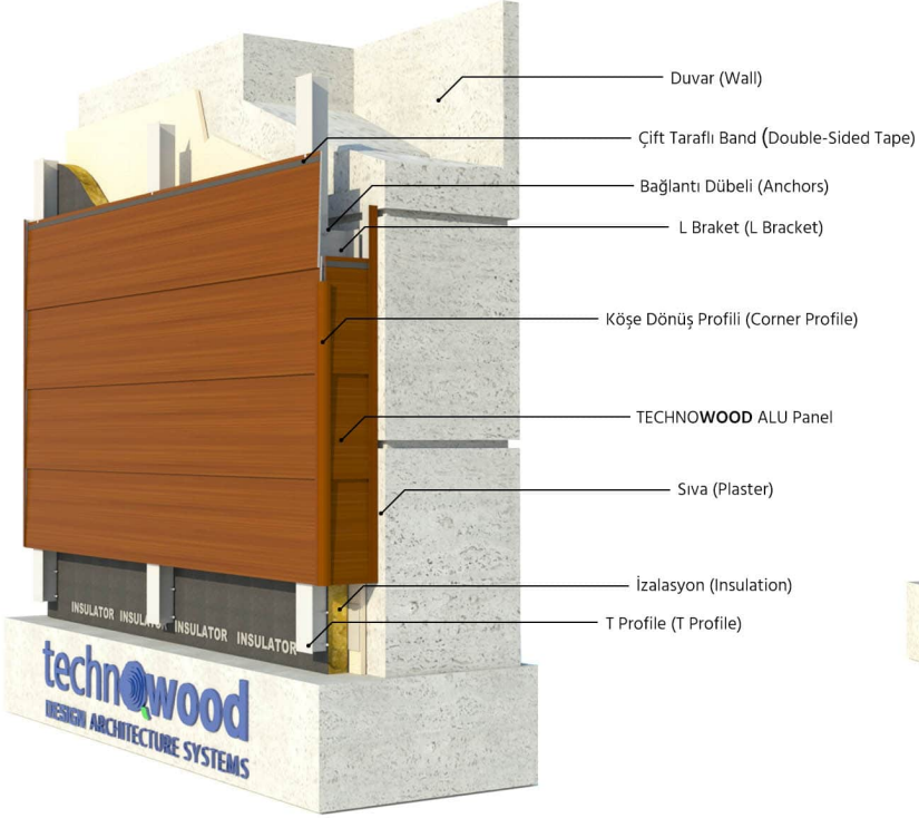
SIDING FAÇADE CLADDING
