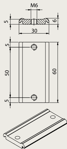
Type LZ.4202 Includes two bolts (M6×16) and locking ring
