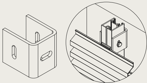
Includes bolt (M6×16), includes nut and locking ring
