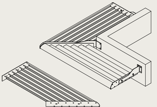
expansion joint on the corner
