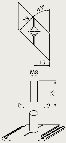
Type LZ.4211 Includes nut M6 and locking ring
